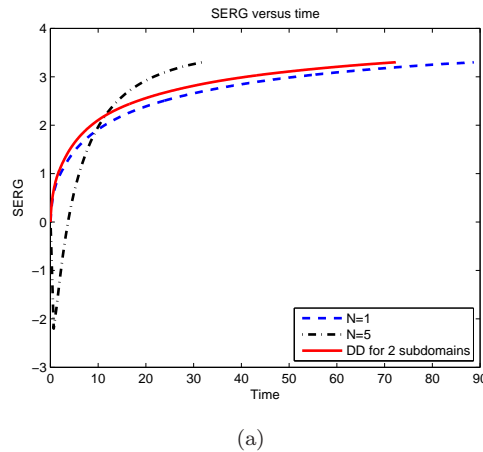
FIG. 6.8. We show for N = 1 , N = 5 of the algorithm in (3.8), and for the domain decomposition algorithm [25] for a decomposition into 2 subdomains the evolution of the quality measure SERG for the deblurring problem of Figure 6.1.
