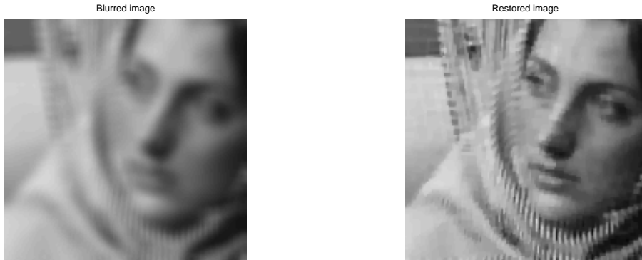
FIG. 6.1. On the left we depict an image, blurred with an averaging kernel of size 9 \times 9 pixels with uniform values 1/81 . On the right we show the corresponding solution computed on 5 orthogonal subspaces by the algorithm in (3.8) with \alpha = \frac{2}{3} \cdot 10^{-4} and stopping criterion (6.2) with S^* = 3.3 .
