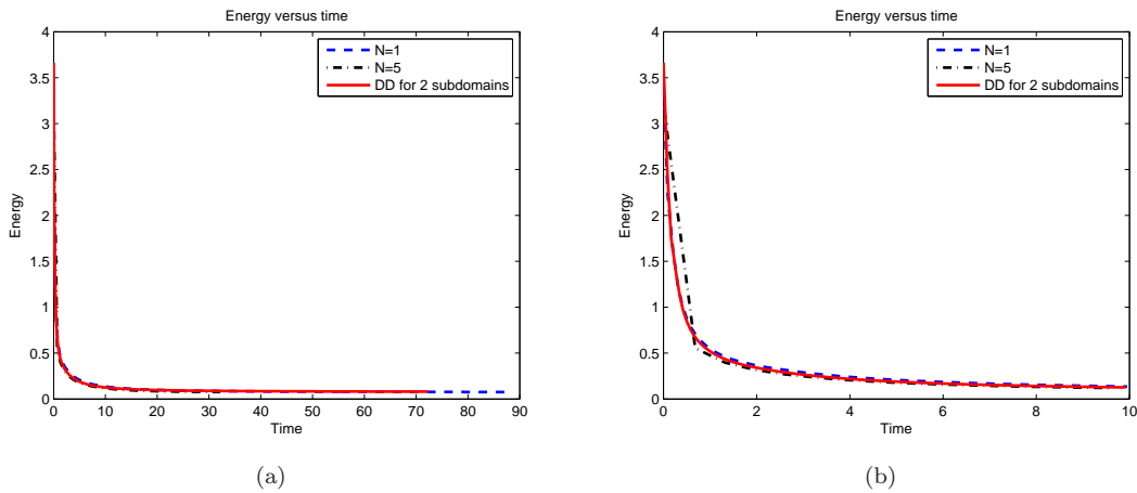
FIG. 6.7. We show for N = 1 , N = 5 , and for the domain decomposition algorithm [25] for a decomposition into 2 subdomains the decay of the energy for the deblurring problem of Figure 6.1. In (b) we zoomed in to the first 10 seconds.
