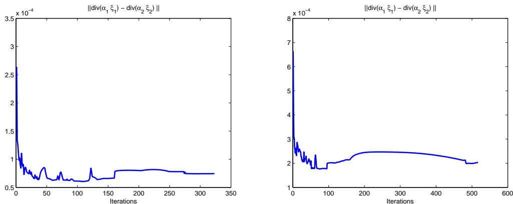
FIG. 6.5. We plot \|\operatorname{div}(\alpha_1 \xi_1^{(n)}) - \operatorname{div}(\alpha_2 \xi_2^{(n)})\| for the problem of Figure 6.1 (left) and Figure 6.6 (right) in view of Lemma 5.1 in order to check whether the algorithm is indeed converging.
