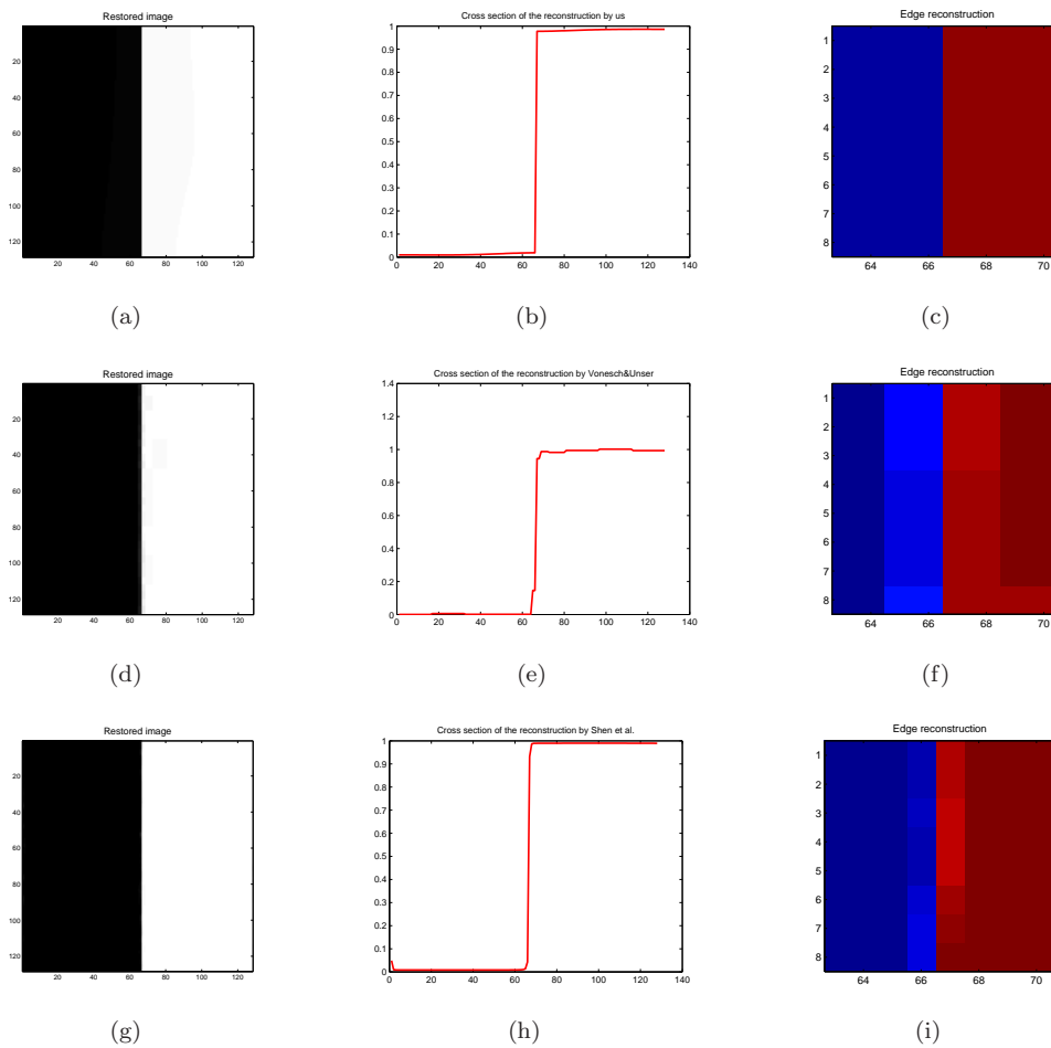
FIG. 6.10. Restoration of the corrupted image in Figure 6.9 with (a) the algorithm in (3.8) with a plot of its cross section in (b); (d) the algorithm by Vonesch and Unser [35] with cross section in (e); (g) the algorithm by Shen et al. [6] with a cross section in (h). In the right column we depict a zoom of the edge where the colors are changed such that dark blue is representing black and dark red is representing white, in order to visualize the edge reconstruction better.
