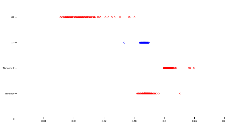
FIG. 5.5. Numerical illustration for the function shaw(100) . The figure presents relative errors (circles) for 100 simulations of y_\delta with 1% noise
