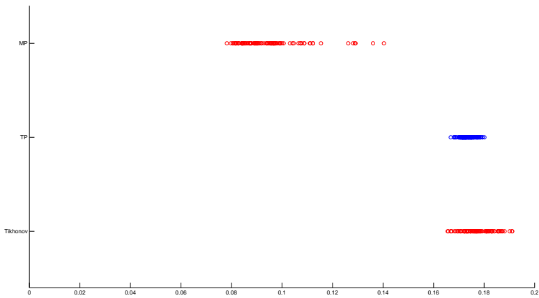
FIG. 5.3. Numerical illustration for the function shaw(100). The figure presents relative errors (circles) for 100 simulations of y_\delta with 1% noise
