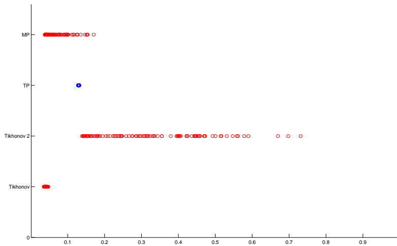
FIG. 5.6. Numerical illustration for the function ilaplace(100, 1) . The figure presents relative errors (circles) for 100 simulations of y_\delta with 1% noise
