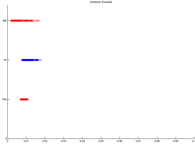
FIG. 5.1. Numerical illustration (first experiment). The figure presents relative errors (circles) for 100 simulations of y_\delta with 1% noise
