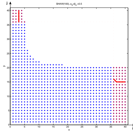
FIG. 5.7. Discrepancy domain and its reconstruction by means of the model function for the function shaw(100) .
