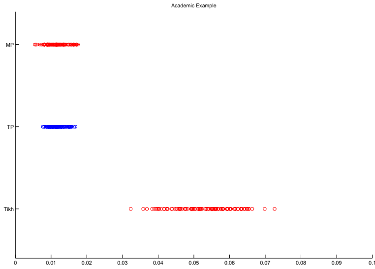
FIG. 5.2. Numerical illustration (second experiment). The figure presents relative errors (circles) for 100 simulations of y_\delta with 1% noise
