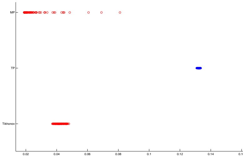
FIG. 5.4. Numerical illustration for the function \text{ilaplace}(100, 1) . The figure presents relative errors (circles) for 100 simulations of y_\delta with 1% noise
